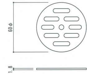
④排水用目皿 (S=1/2)
