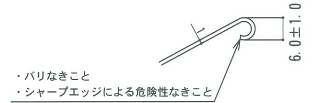
B部拡大 1/1
