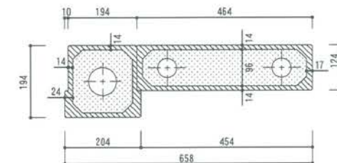
C'-C断面図
