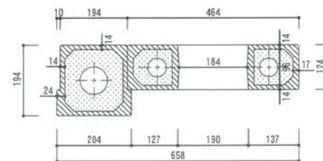
C'-C断面図
