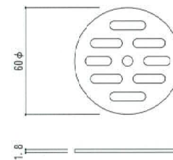
④排水用目皿 (S=1/2)
